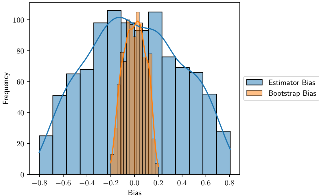
Distribution of Bias_Brain_Amygdala
